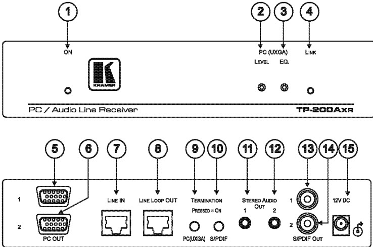
Figure 2: TP-200AXR PC / Audio Line Receiver
