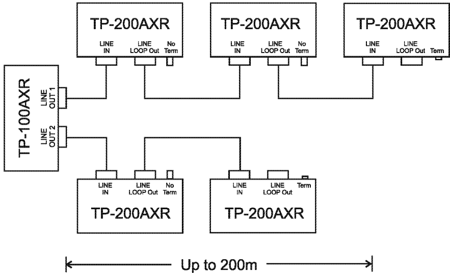
Figure 4: Connecting Multiple Devices
