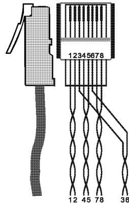
Figure 5: CAT 5 PINOUT
