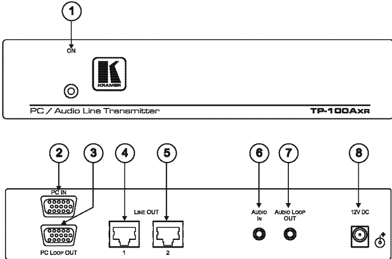
Figure 1: TP-100AXR PC / Audio Line Transmitter
