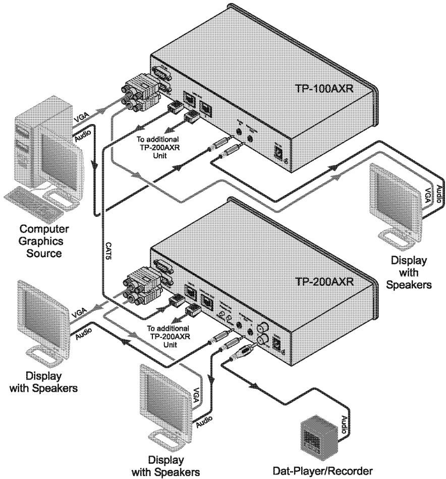
Figure 3: Connecting the PC / Audio Line Transmitter / Receiver System
