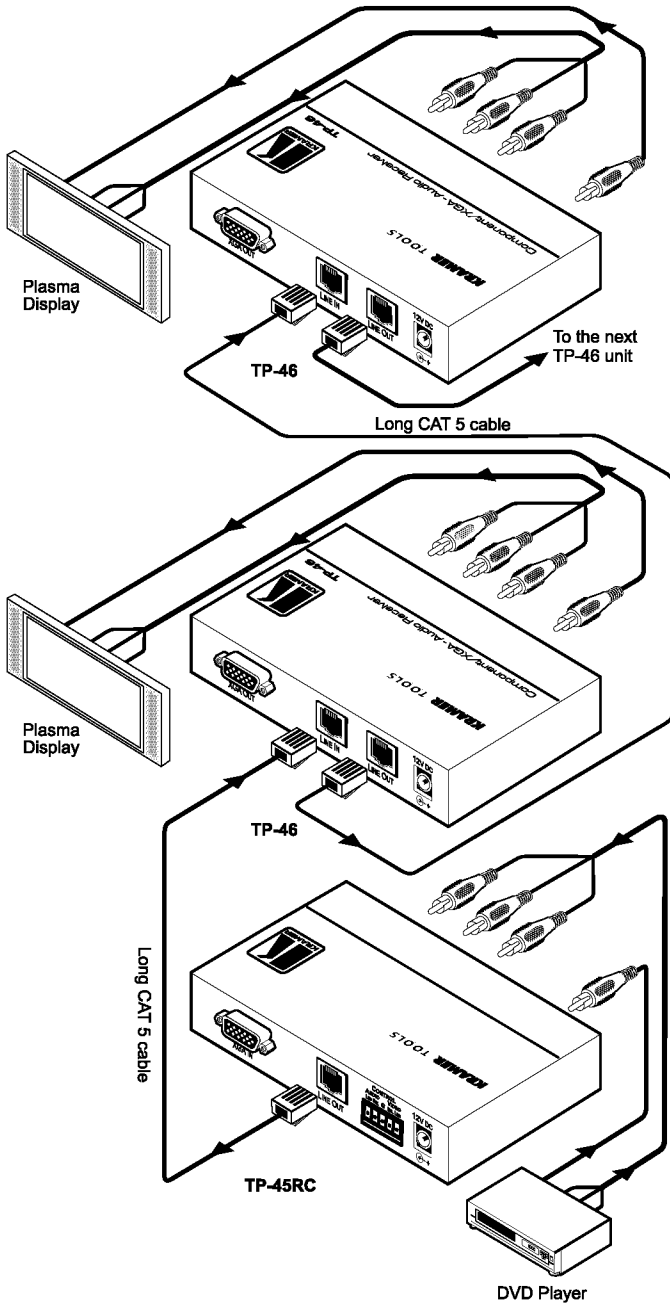
Figure 7: Component/XGA – Audio Distribution System, Component Video Mode
