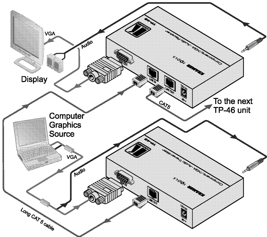
Figure 6: Component/XGA – Audio Distribution System, XGA Mode
