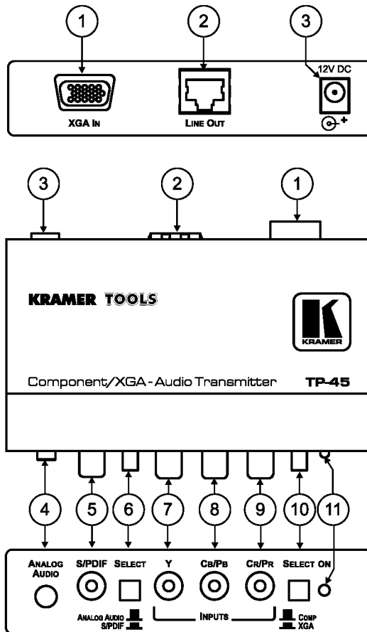
Figure 1: TP-45 Component/XGA – Audio Transmitter
