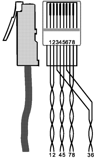
Figure 9: CAT 5 PINOUT
