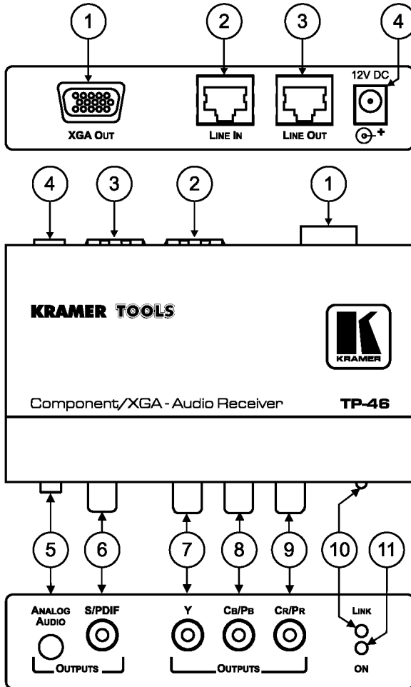
Figure 4: TP-46 Component/XGA – Audio Receiver
