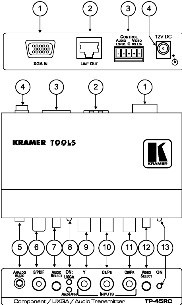
Figure 3: TP-45RC Component/XGA – Audio Transmitter
