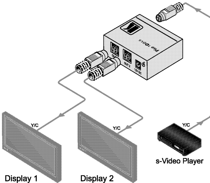
Figure 4: Connecting the PT-102SN 1:2 s-Video DA
